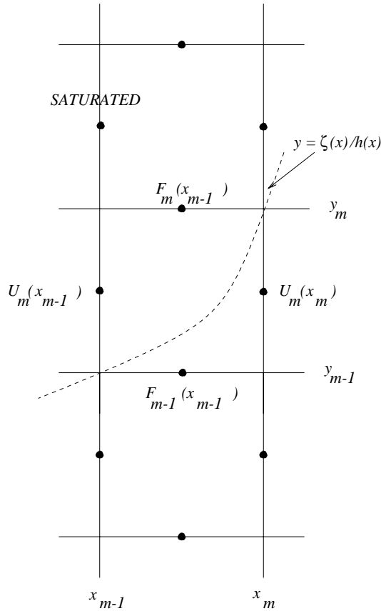
FIGURE 5. Numerical grid near saturation boundary.
